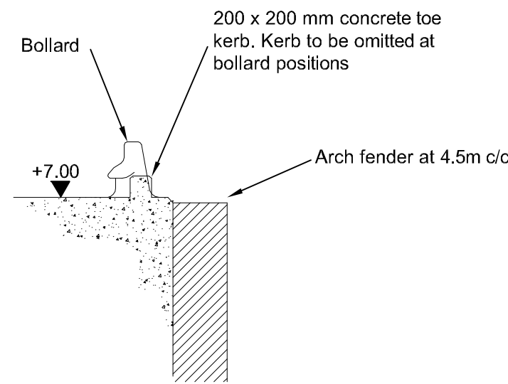
Deep Water Quay Toe Kerb Detail 1:50
